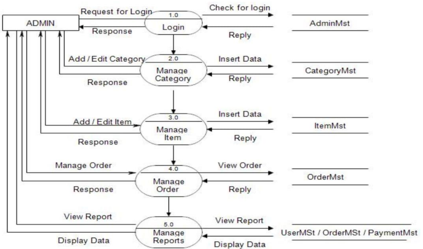
Admin Side DFD - 1st Level
